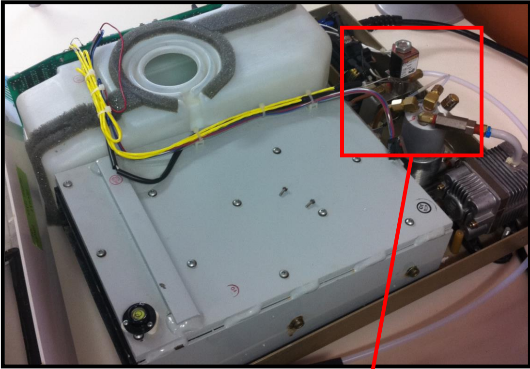
Statim unit with cover removed (Statim 2000 unit shown, 5000 model will look slightly different)
